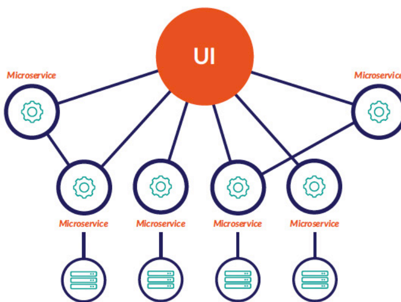
Microservice Architecture
